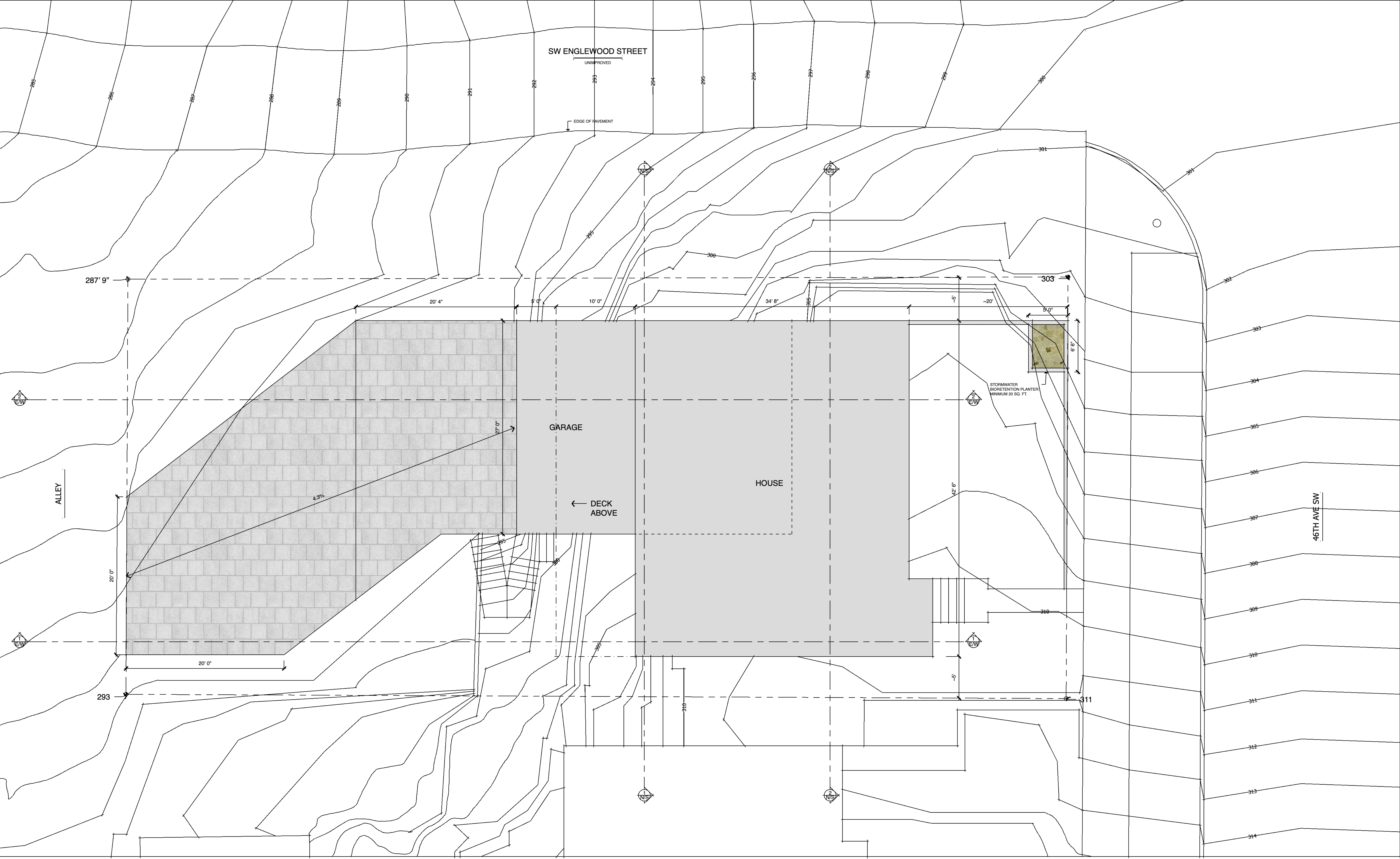
PRELIMINARY SITE PLAN: 5303 46 AVE SW NORTH NTS
