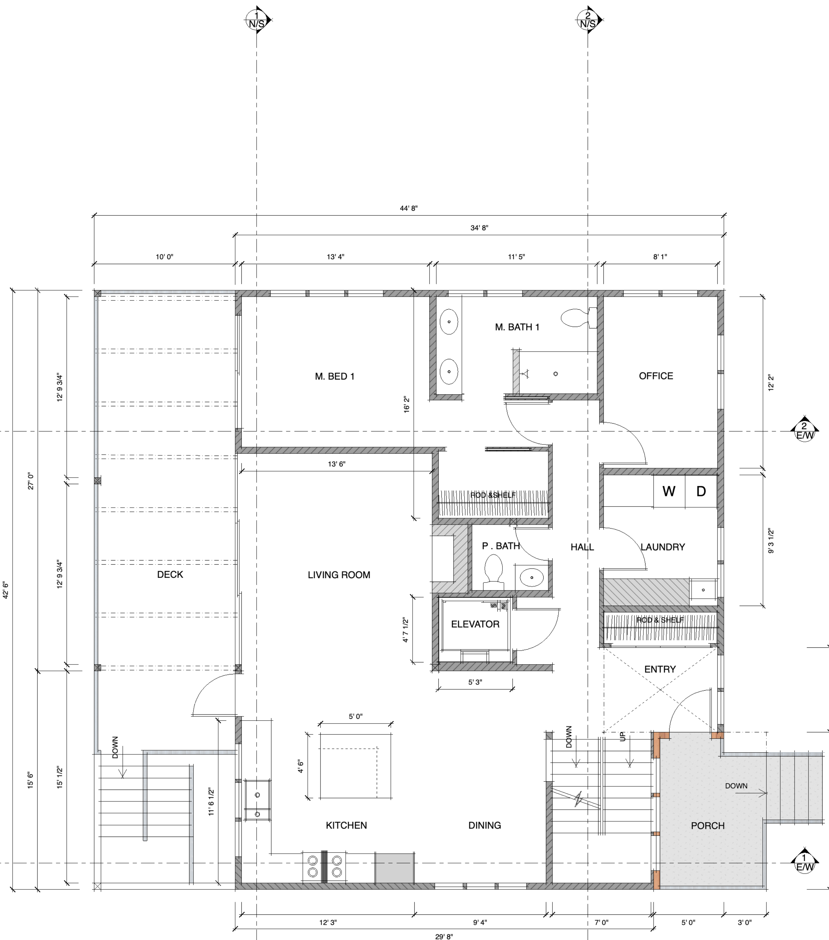
MAIN PLAN NORTH 1/4" = 1' 0"
