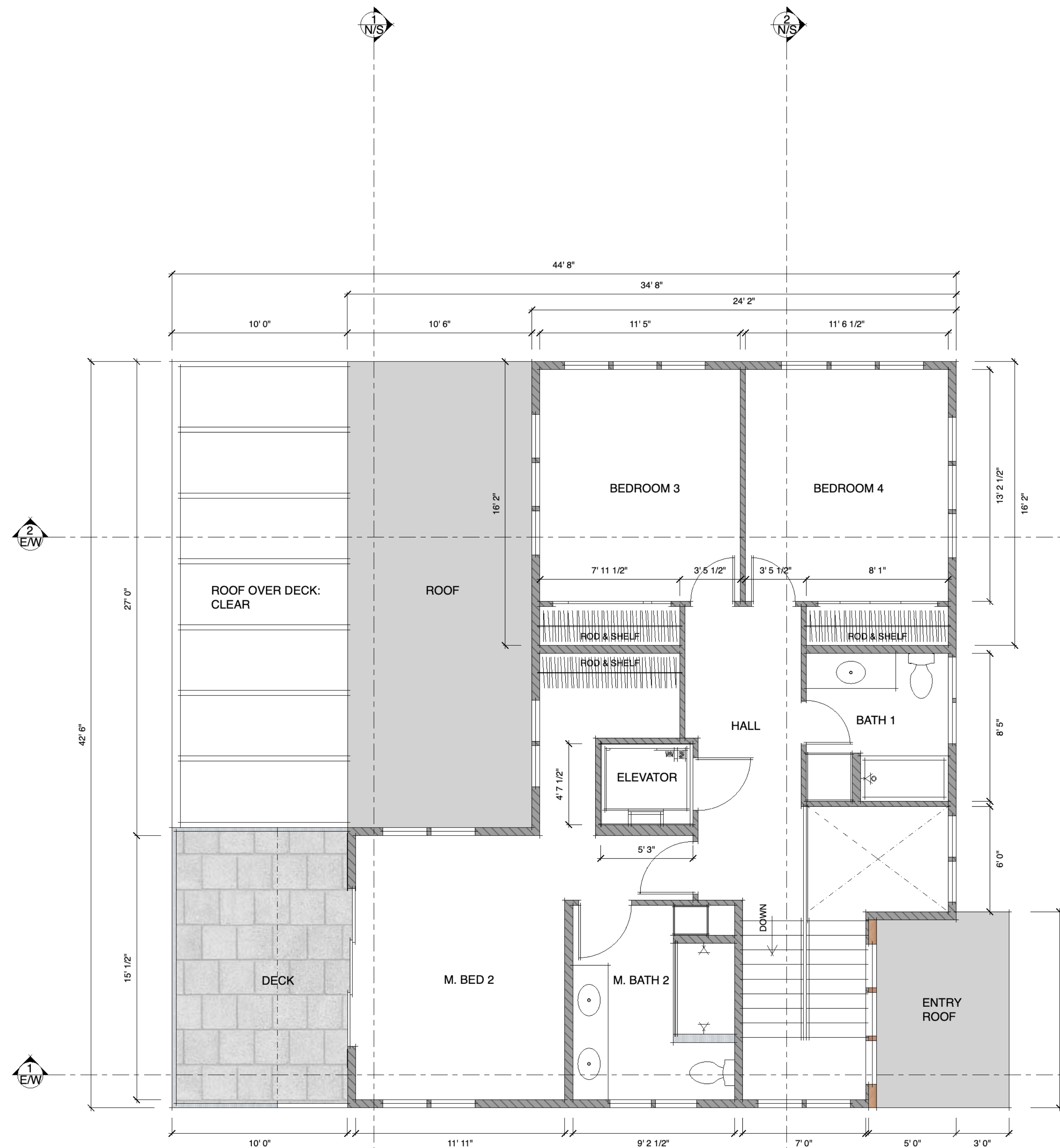
UPPER PLAN NORTH 1/4" = 1' 0"
